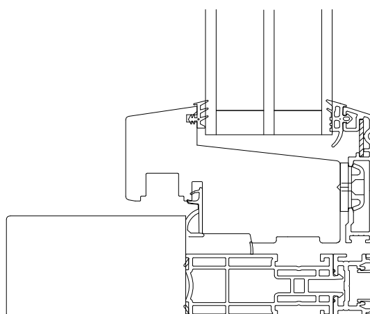
Triple Glazing (U-value = 0,5 w/m2k)
